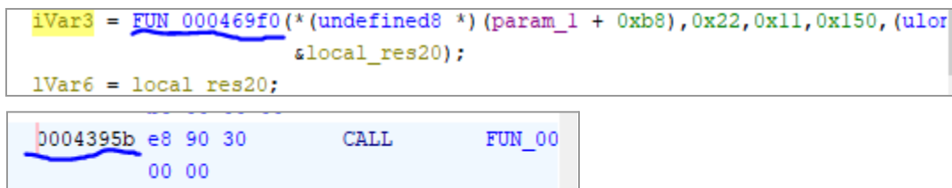
Figure 2 — IoCreateDevice reference in Ghidra.
